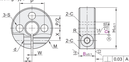
Three-Hole Locking Type
