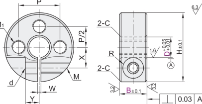
Three Threaded Hole Locking Type
