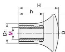
Internal Thread Type
