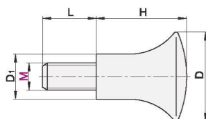
External thread type
