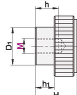
Internal Thread Type
