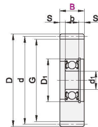
Single Bearing
