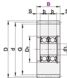
Double Bearing
