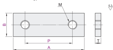
Double Hole Type
