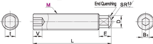
Hex Socket with Wrench Slot Type
