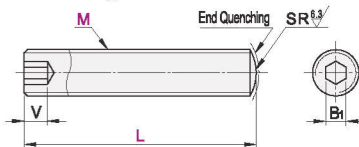
Hex Socket Type
