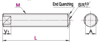
Wrench Slot Type
