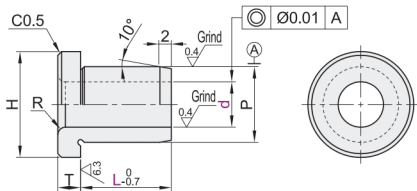
Shouldered Type, Standard Type
