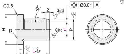
Shouldered Type, Thin-walled Type
