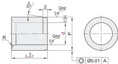
Shouldered Type, Standard Type
