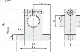
T Type
