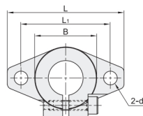
Flange Type
