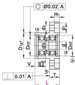
Round Flange Type
