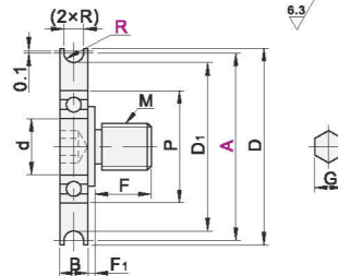
External thread type
