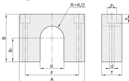
Standard Type
