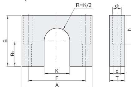
Thin-wall Type
