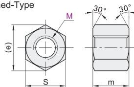
Thickened-Type
