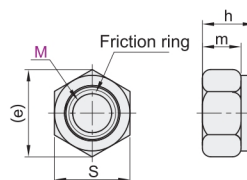
Non-Metallic Insert Hex Locknuts
