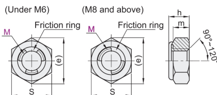
All-Metal Locknuts
