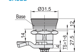
Wing-shaped Lock Head CASBD
