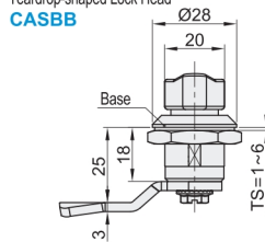
Teardrop-shaped Lock Head CASBB
