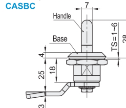
Umbrella-shaped Lock Head CASBC
