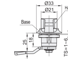
Lock Head with Hook CASCO
