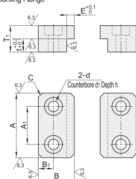
Single Piece Mounting Flange
