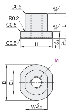
Cylinder Connector Internal Thread
