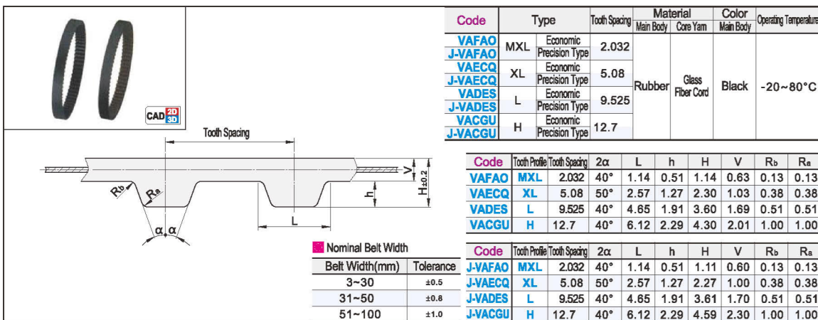
VAFAO-MXL (Tooth Spacing: 2.032)
