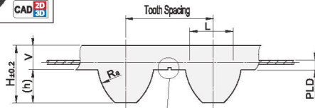
■ J-VBHAL-S2M (Tooth Spacing: 2)
