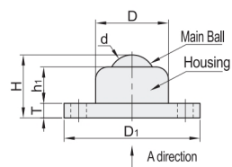
With Drain Hole Type
