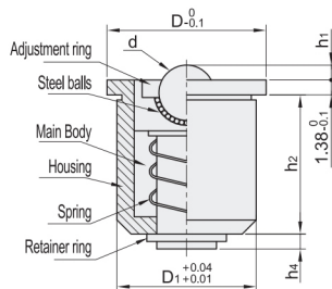
Plunger Type
