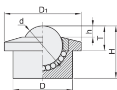
Semi-Press-in Type
