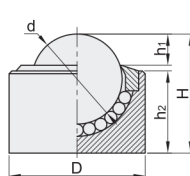
Full Press-in Type
