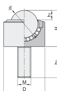
Screw Type
