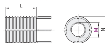
④ Standard Type.Fine Thread
