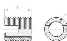
Self-tapping Slotted Type
