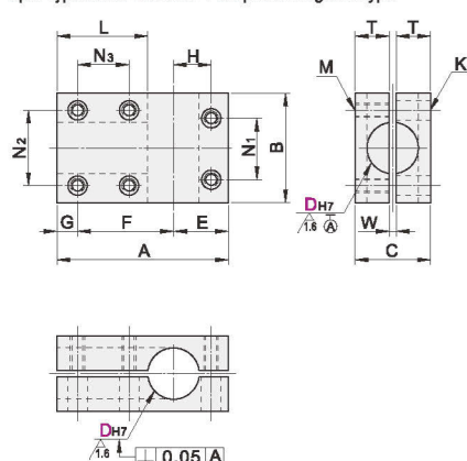
Split-Type Same Diameter T-shaped Orthogonal Type
