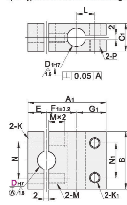
Split-Type Different Diameter Orthogonal Type
