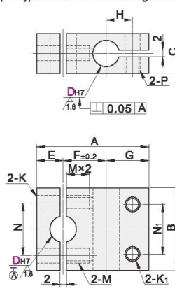
Split-Type Same Diameter Orthogonal Type
